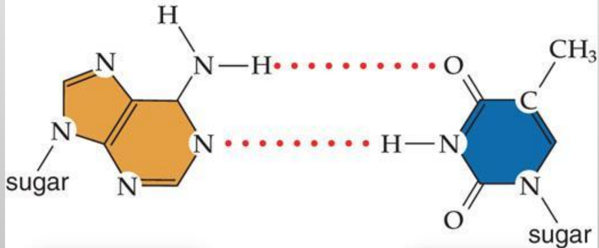
adenine (A)
