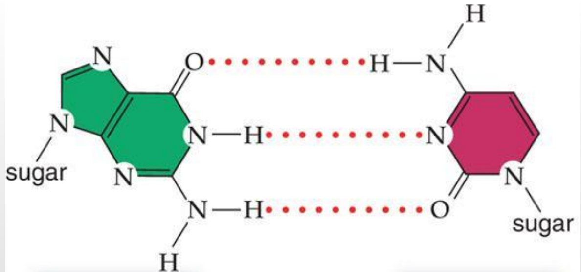
guanine (G)
