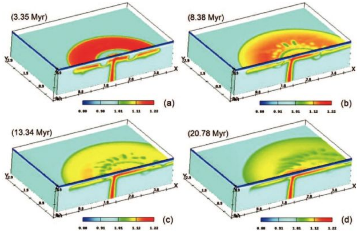
Figure 2. Temperature distribution (a-d) at different times for the model without a lithospheric root. Horizontal slice is at a depth of 139 km.
