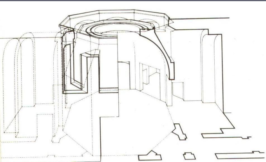
ROME. OCTAGONAL VAULTED HALL IN THE DOMUS AUREA, PERSPECTIVE PLAN (after W. L. MacDonald)
