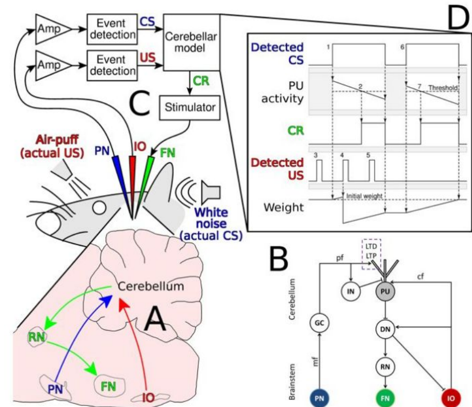
Figure 1: System overview.
