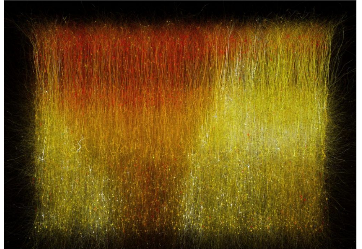
Simulation of neural activity in a tissue slice (©Blue Brain Project / EPFL ©2005 – 2019. All rights reserved.)
