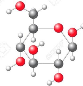
β-D-Glucose (cyclic)
