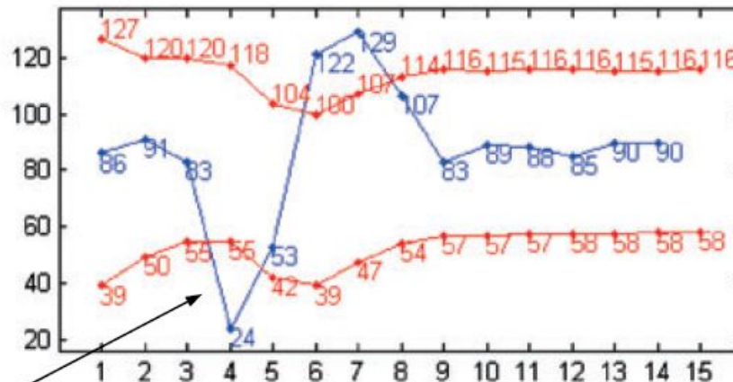
OFF Score
