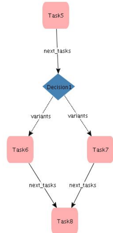
Sequential execution
