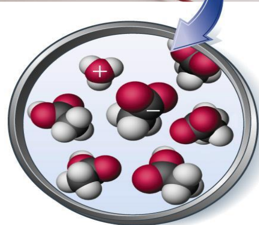
(c) 1 M \text{CH}_3\text{COOH}(\text{aq}) Weak electrolyte Solute consists mostly of molecules; some ions:
