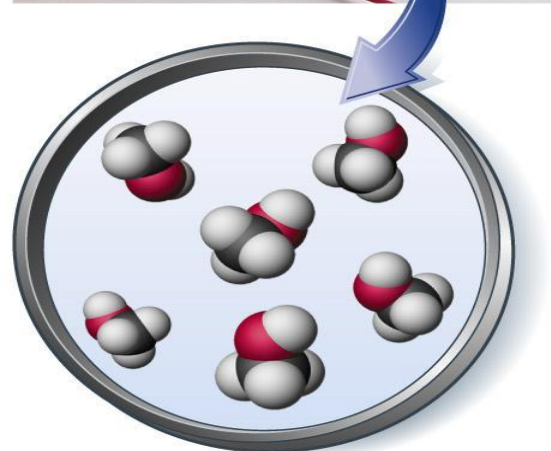
(a) 1 M \text{CH}_3\text{OH} Nonelectrolyte Solute consists of molecules; no ions
