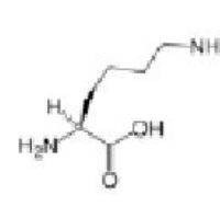
L-Lysine
