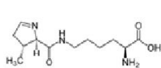
L-Pyrrolysine
