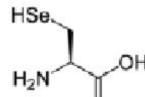
L-Selenocysteine
