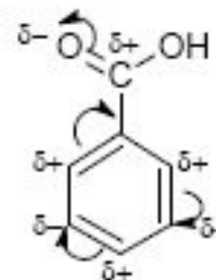
COOH: -М
