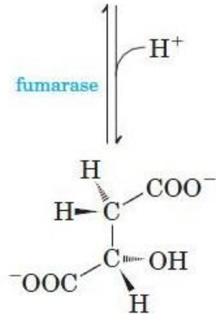
Malate
