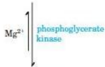
1,3-Bisphosphoglycerate
