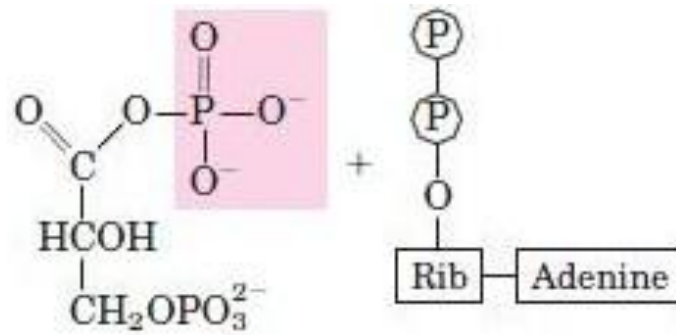
1,3-Bisphosphoglycerate
