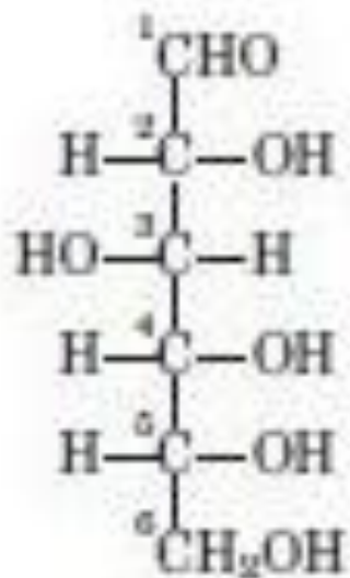
D-Glucose
