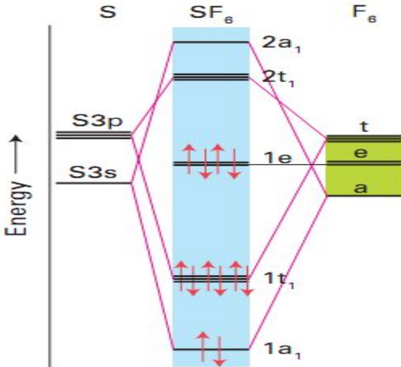
Fig. 2.31 A schematic molecular orbital energy level diagram for SF_6 .
