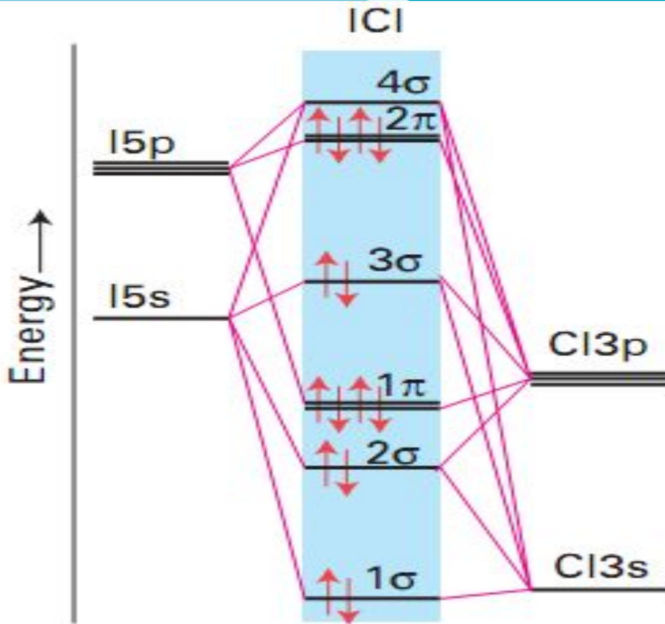
Fig. 2.24 A schematic illustration of the energies of the molecular orbitals of ICl.
