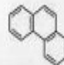
Phenanthrene C_{14}H_{10}
