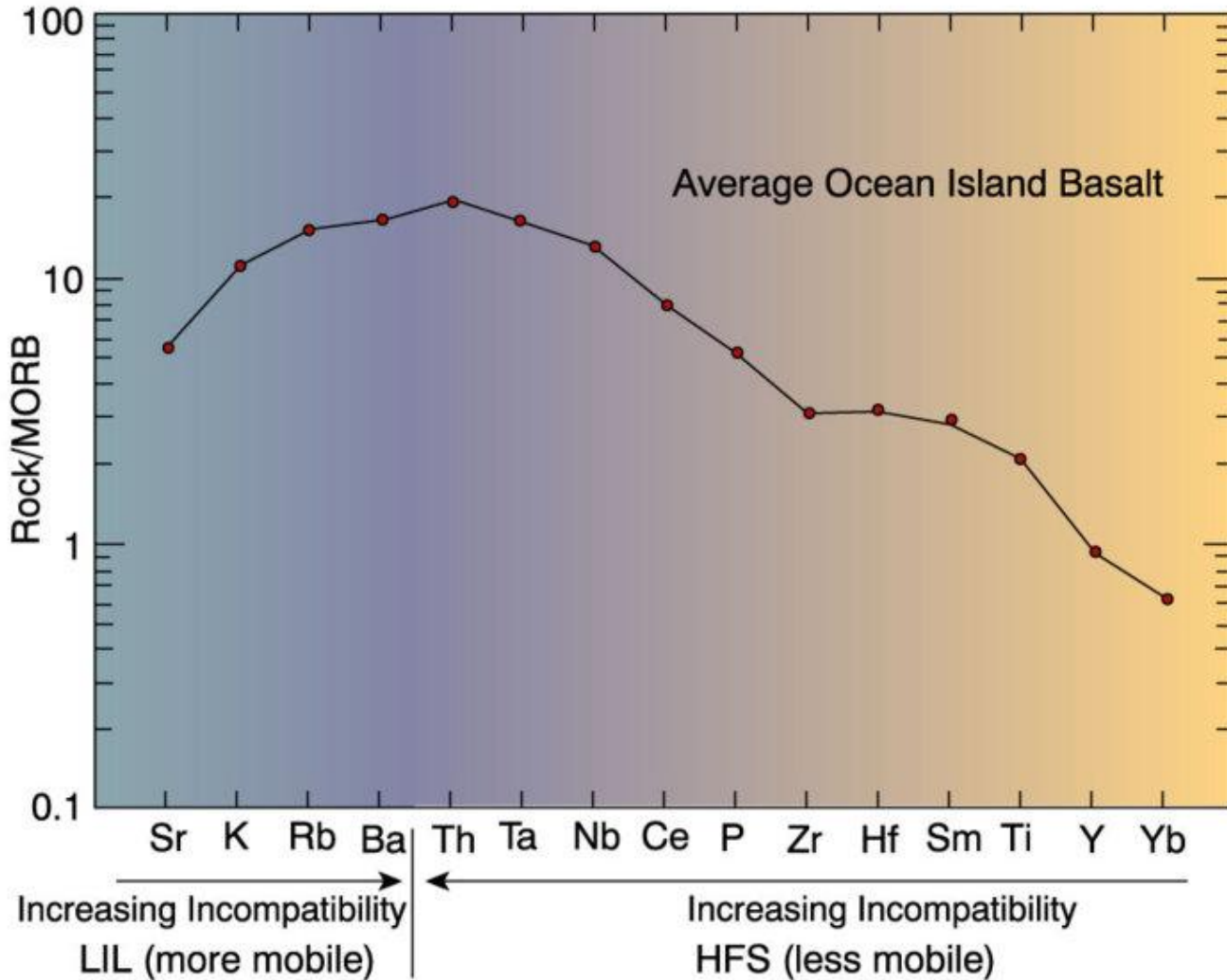
Figure 9-7. Ocean island basalt plotted on a mid-ocean ridge basalt (MORB) normalized spider diagram of the type used by Pearce (1983). Data from Sun and McDonough (1989). From Winter (2001) An Introduction to Igneous and Metamorphic Petrology. Prentice Hall.
