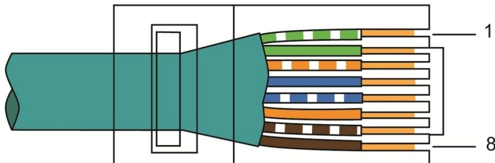
EIA/TIA-568A
