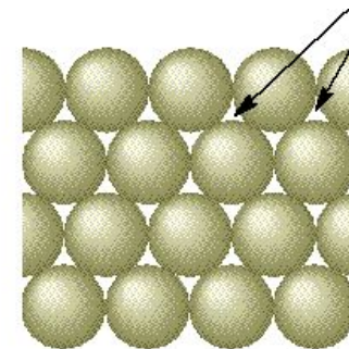
Sandstone porosity
