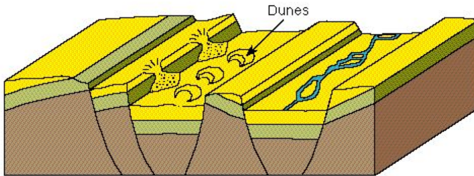
Continental deposition
