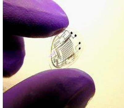
Flexible electronics embedded in contact lens
