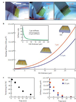
Figure 2 | Time-dependent change in the silk substrate devices. a, Dissolution of the silk through submersion in warm water. b, Total bending stiffness \mu\text{m} and 2.5 \mu\text{m} electrochromic area encompassing silk film, as a function of the thickness of the supporting silk film, base. The ratio of bending stiffness between 7 \mu\text{m} and 2.5 \mu\text{m} . c, Time-dependent change in the volume of a silk film during dissolution (left frame) and bending stiffness calculated for silk film and 100% ethanol for 5 h for two different area thicknesses (right frame). The 5 h ethanol treatment increases the dissolution time from minutes to 48 h.
