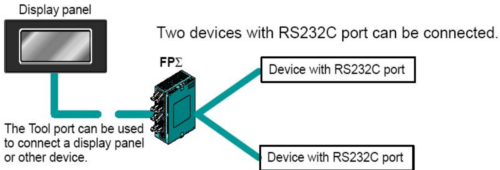
Figure 1: Features-communication (RS232C)
