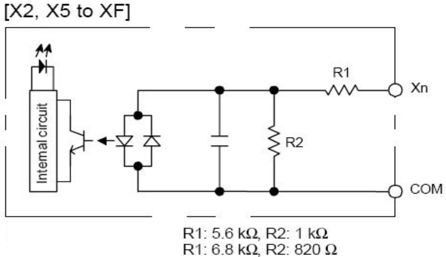
FP \Sigma Internal circuit diagram (Input-2)
