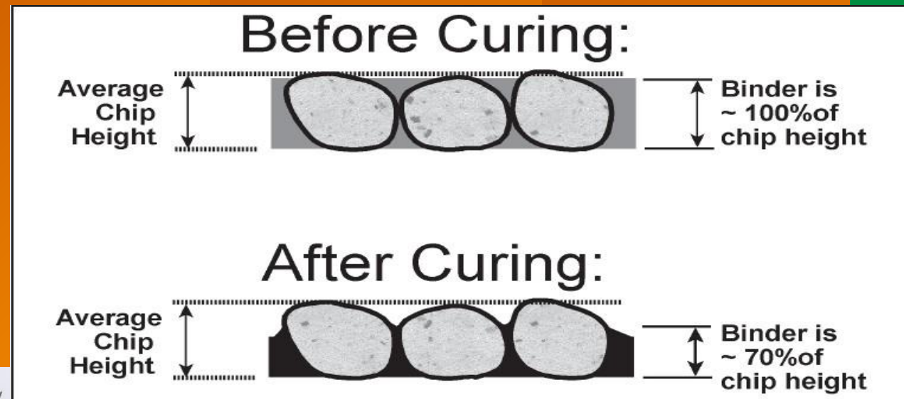
Figure 4.2. Change in volume after emulsion has cured
