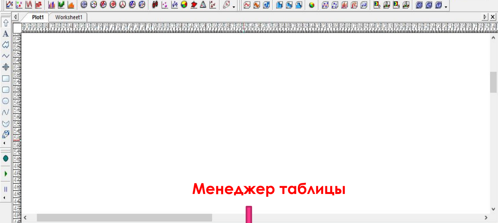
Worksheet Manager
