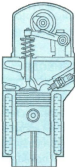
OHV/OHC
