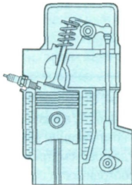
OHV
