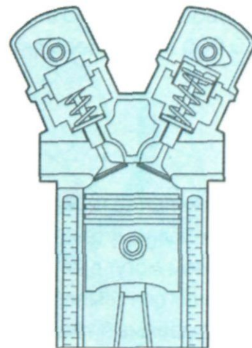
OHV/DOHC
