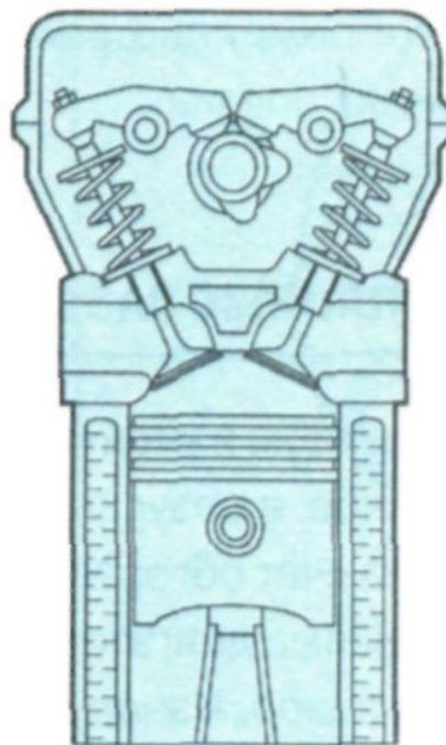
OHV/OHC
