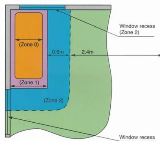
Bath Tub (plan)
