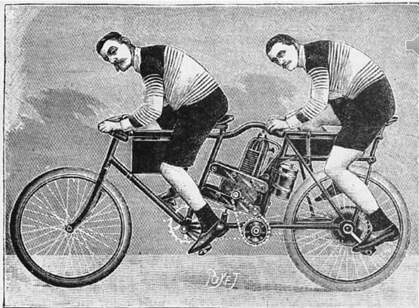
FIG. 6.—MM. COURET AND BOUDIN UPON A GASOLINE TANDEM BICYCLE.
