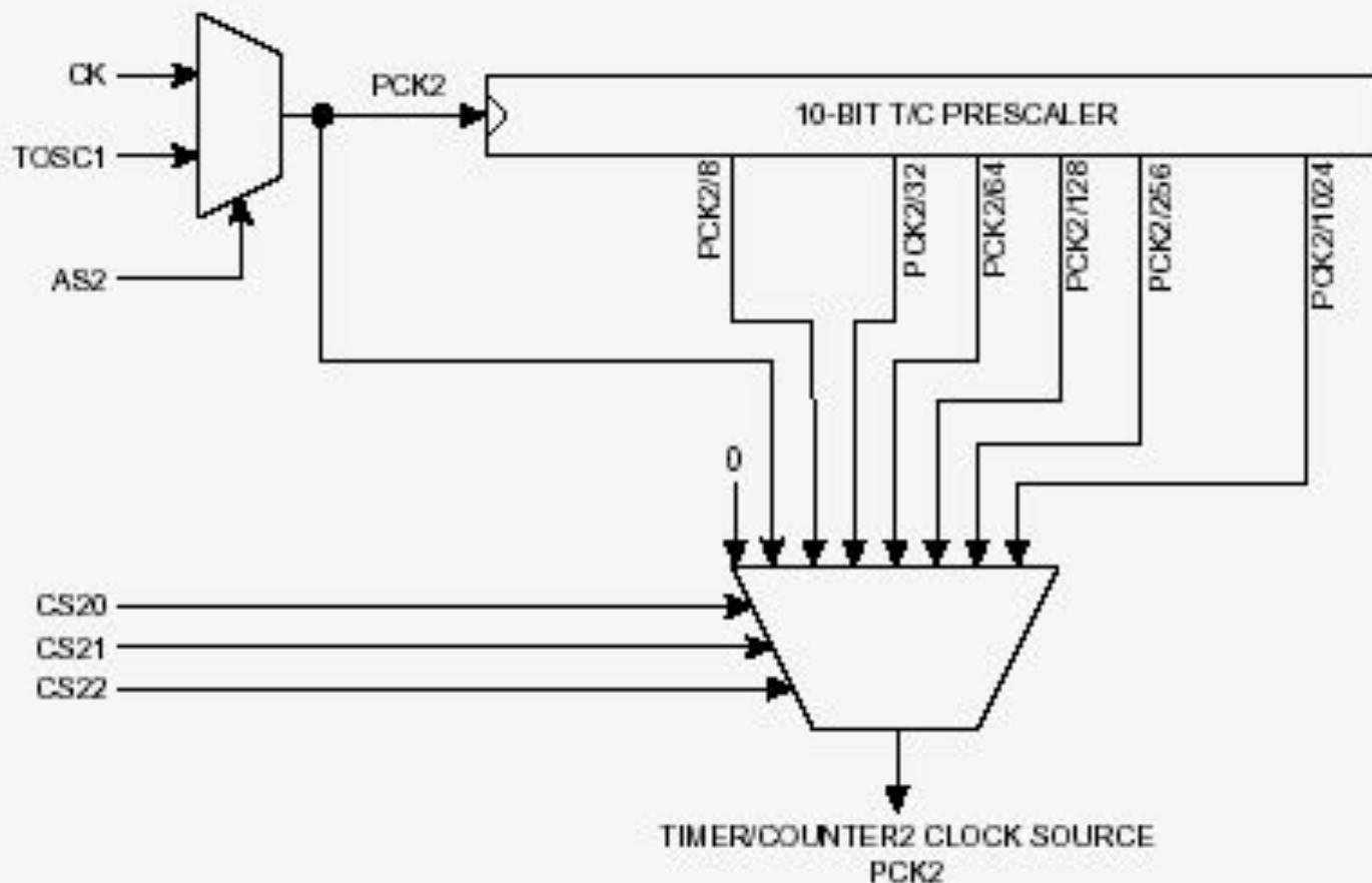
Timer/Counter 2 Prescaler
