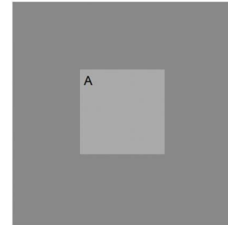
Contrast induction
