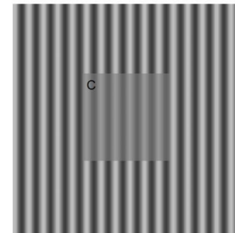
Contrast supression
